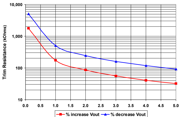
Figure C: Trim Graph for 1.65Vout module
