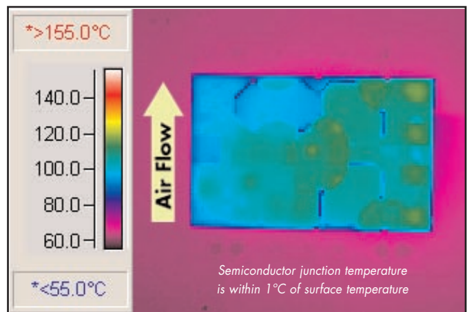
Figure 6: Thermal plot of converter at 40 amp load current with 55°C air flowing at the rate of 200 LFM. Air is flowing across the converter from pin 3 to pin 1 (nominal input voltage).
