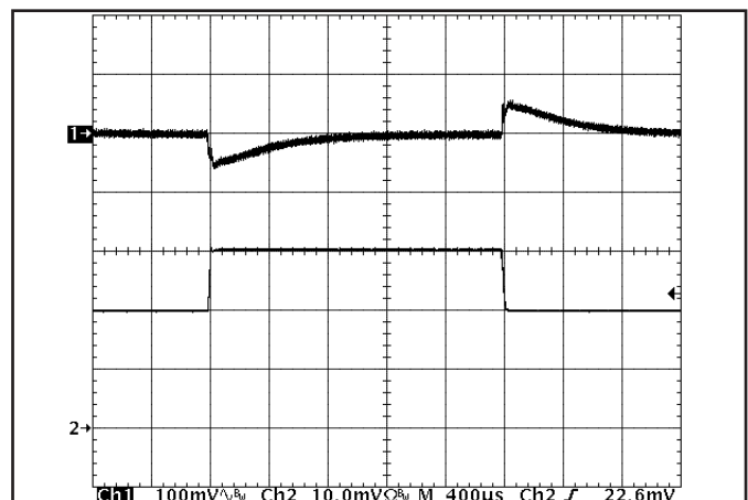
Figure 12: Output voltage response to step-change in load current (50%-75%-50% of I_{out(max)} ; dI/dt = 1\text{A}/\mu\text{s} ). Load cap: 470μF, 30 mΩ ESR tantalum capacitor and 1μF ceramic cap. Ch 1: V_{out} (100mV/div), Ch 2: I_{out} (10A/div).
