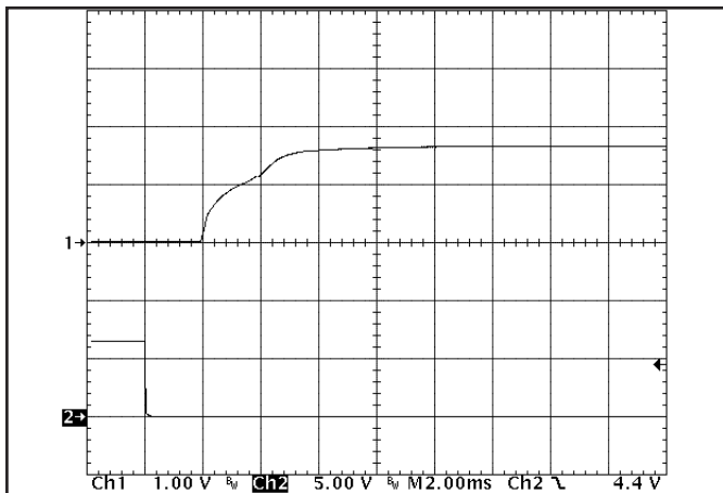
Figure 9: Turn-on transient at full rated load (resistive load) (2 ms/div). Input voltage pre-applied. Ch 1: V_{out} (1V/div). Ch 2: ON/OFF input (5V/div)
